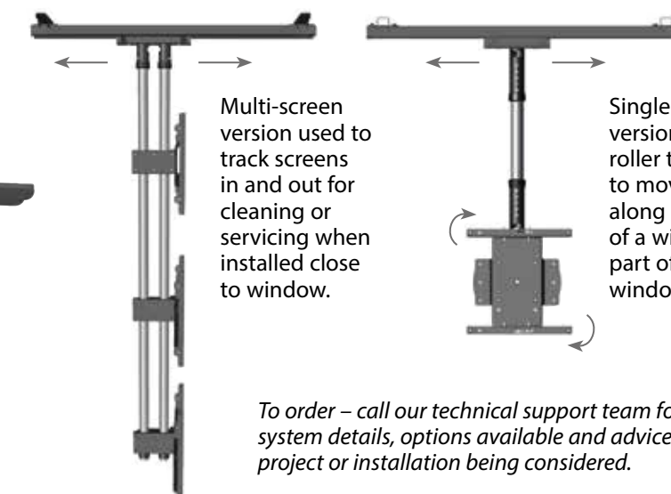
Typical roller track in window display use
