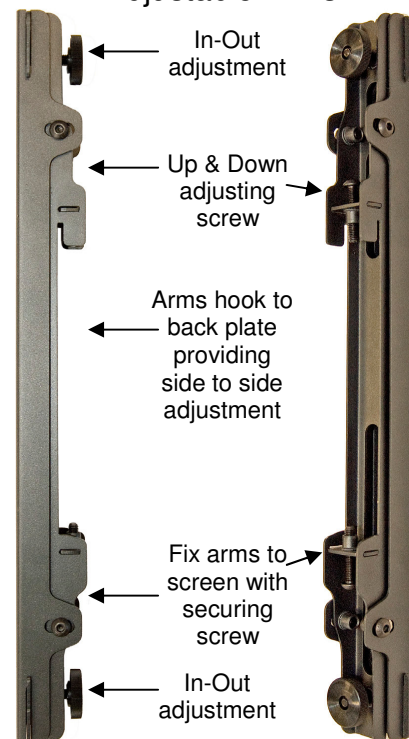
WALL MOUNTED CLOSED POSITION *600 x 400 – 85mm 800 x 400 – 130mm
